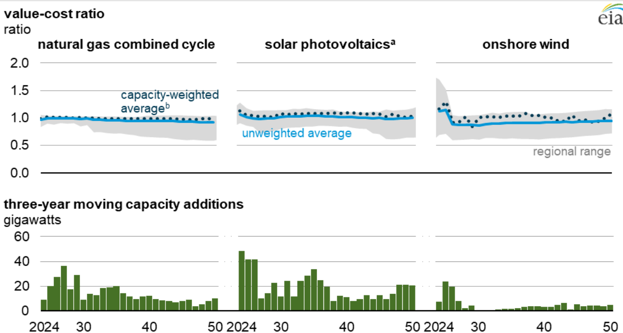
Figure 5. Value-cost ratio and three-year moving capacity additions for selected generating technologies, 2024–50
